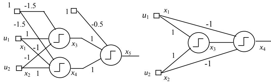
Figure 1.9. Two different implementations of the exclusive-or function by using artificial neurons
