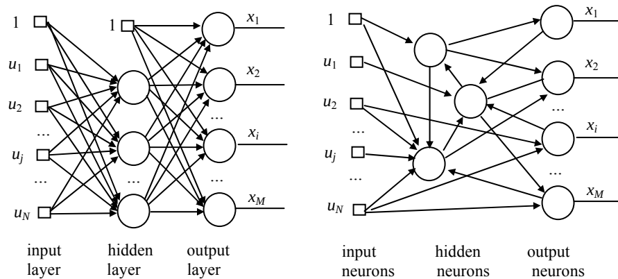
Figure 1.10 a) layered feedforward neural network b) nonlayered recurrent neural network
