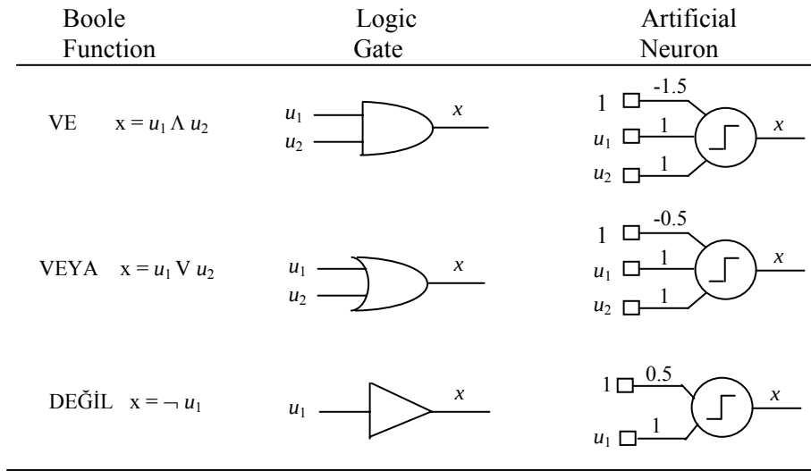
Figure 1.8. Implementation of Boolean functions by artificial neuron
