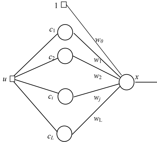
Figure 9.4 Single input, single output RBF network
